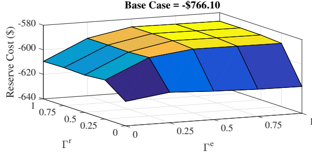
Fig. 7. Reserve cost for different risk aversion values
