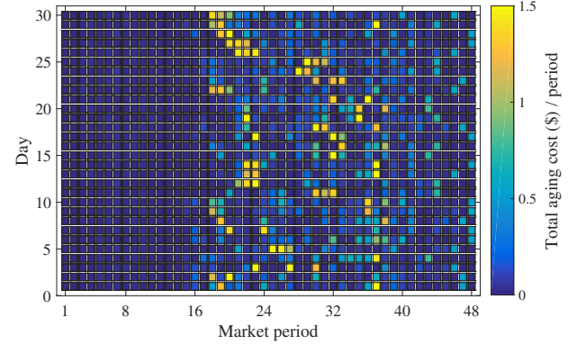
(a) Base case without aging constraints
